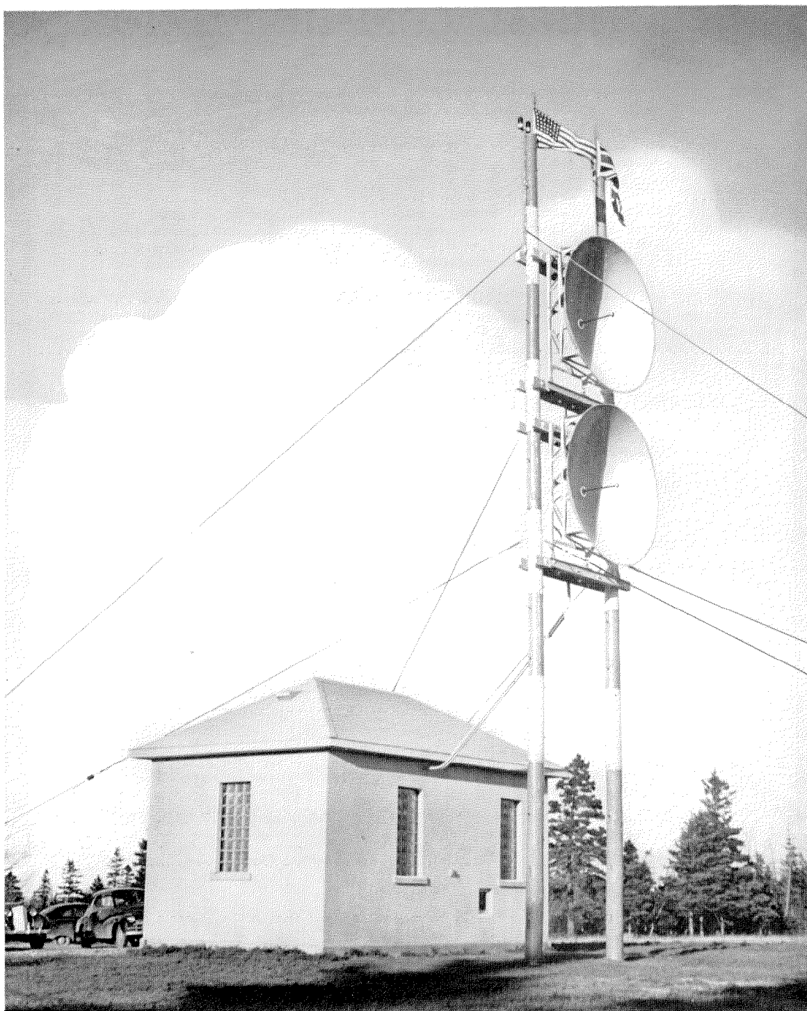
This microwave radiotelephone terminal at Fraser's Mountain near New Glasgow, Nova Scotia, together with a similar installation at Tea Hill, Charlottetown, Prince Edward Island, provide 23 telephone circuits across Northumberland Strait, noted for the ability of its winter storms in breaking submarine cables. The first commercial installation of its kind in the world, this 46-mile 2000-megacycle link uses pulse-time modulation. It was constructed for the Maritime Telephone and Telegraph Company of Halifax and the Island Telephone Company of Prince Edward Island by Federal Electric Manufacturing Company of Montreal, Canada.
